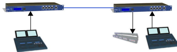
Illustration 5: IP Merging
